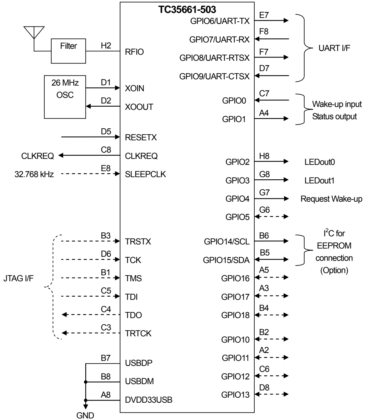
Figure 2-1 TC35661-503 System Configuration Example
