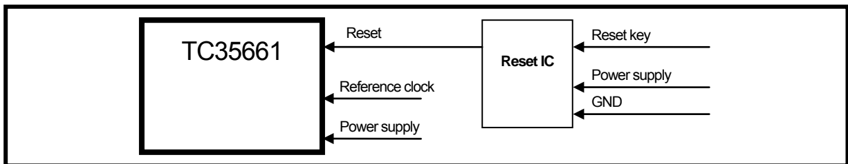
Figure 4-1 Reset IC connection example
