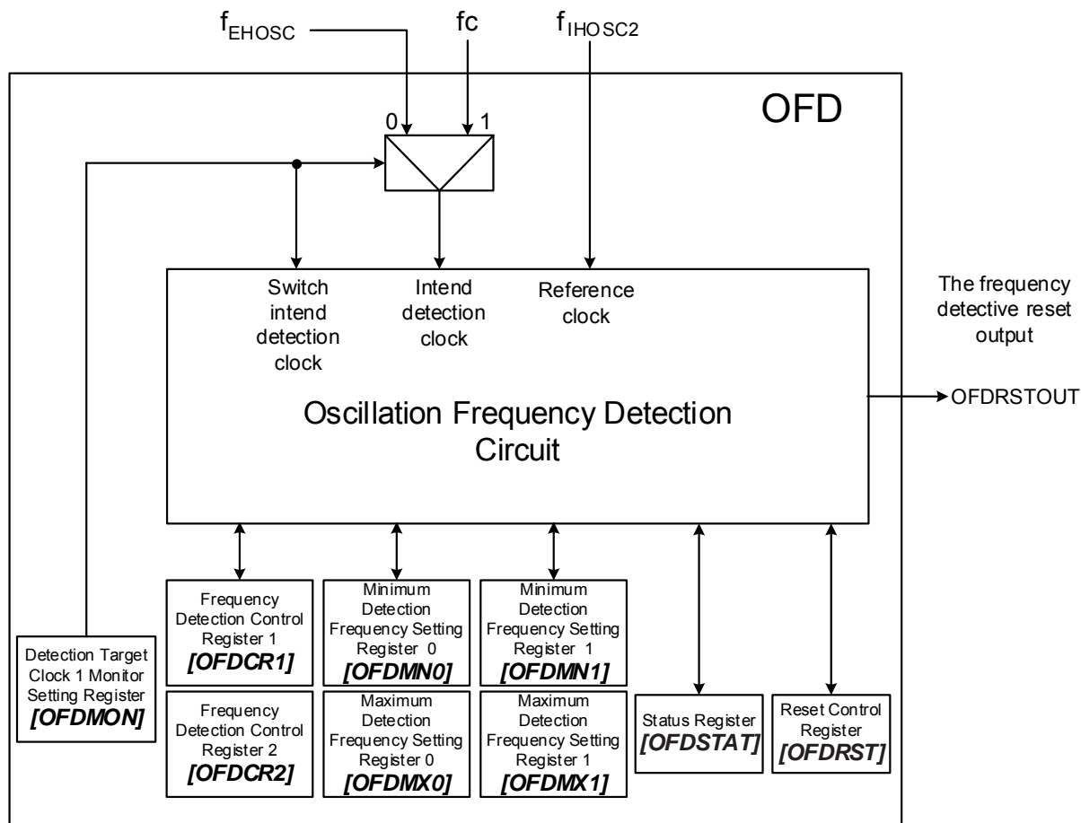
Figure 2.1 Oscillation Frequency Detector Block diagram
