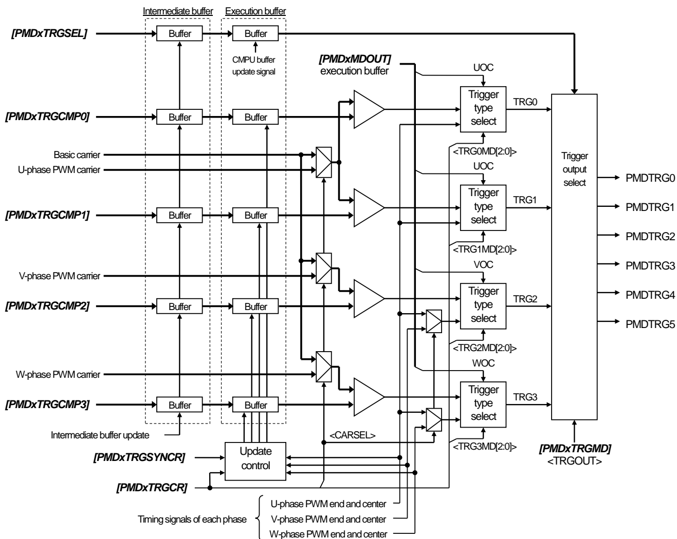
Figure 3.15 Synchronous trigger generation circuit
