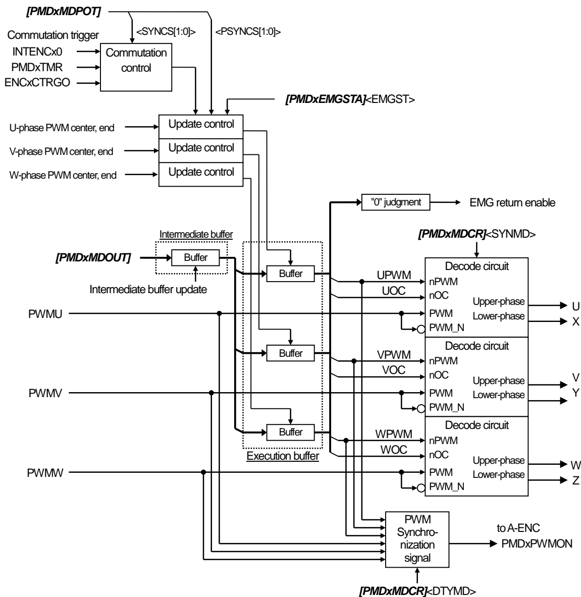
Figure 3.7 Conduction control circuit
