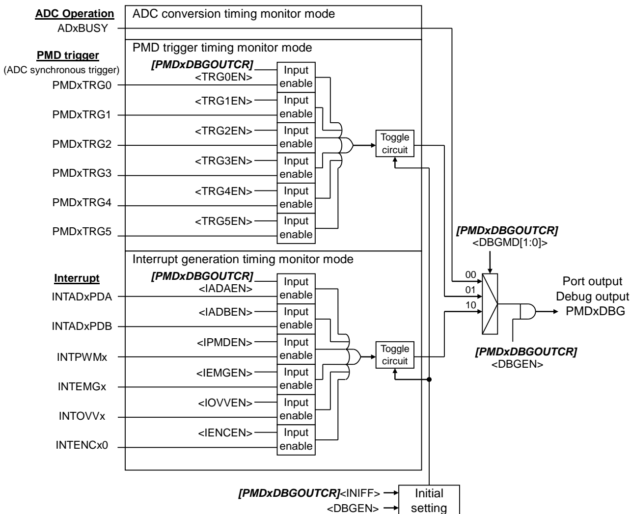
Figure 3.19 Debug output circuit
