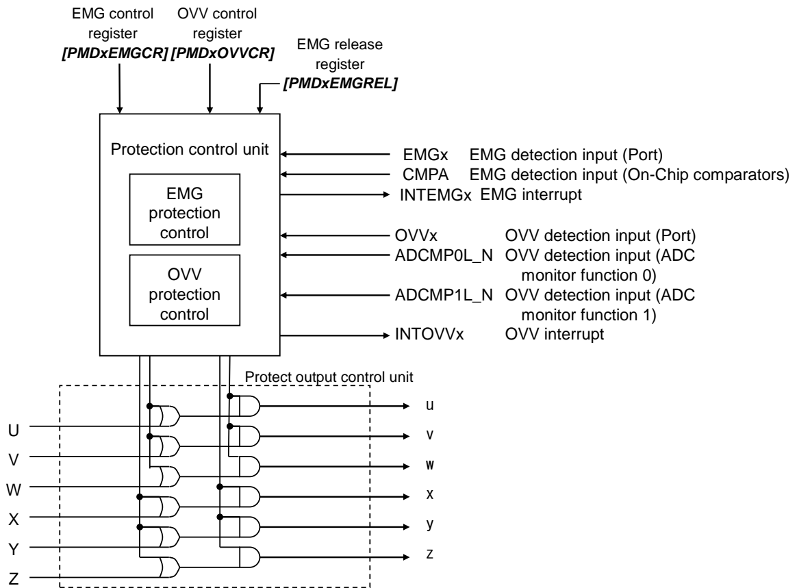
Figure 3.8 Protection control circuit
