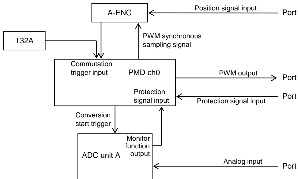
Figure 1.1 Connection diagram of PMD and peripherals
