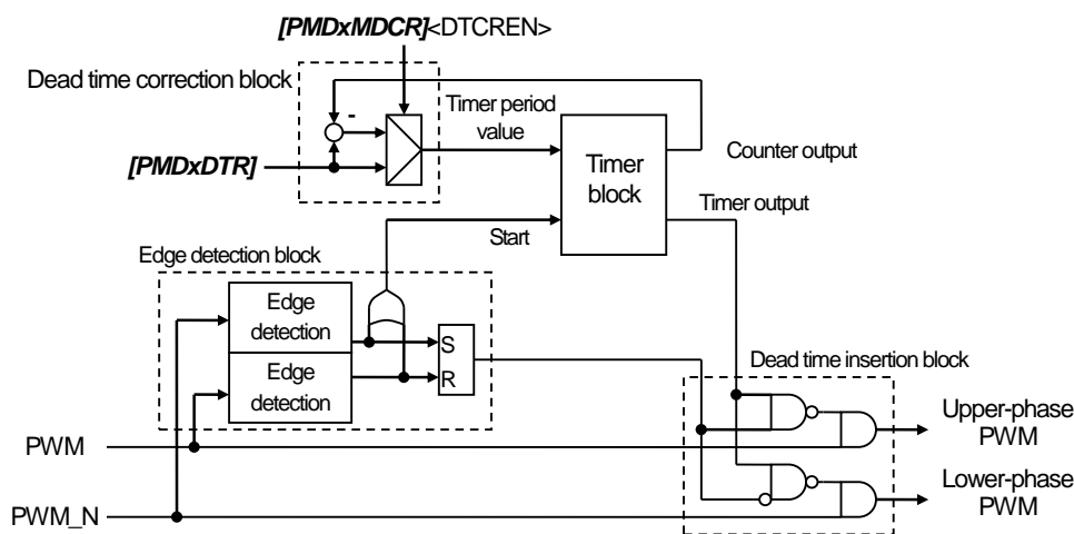
Figure 3.12 Dead time circuit
