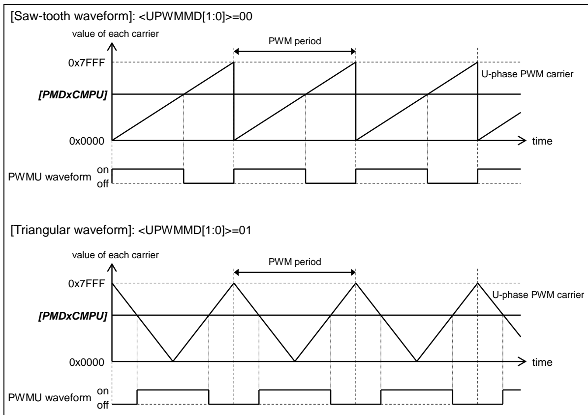
Figure 3.6 PWM waveform
