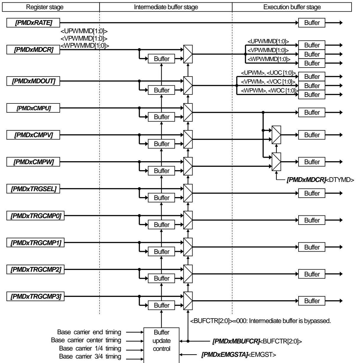
Figure 3.17 Register buffer configuration
