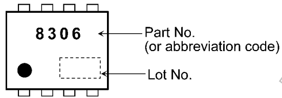
Fig. 7.1 Marking
