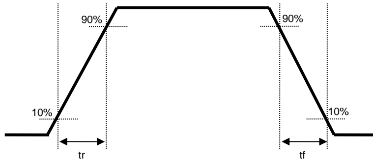
Figure 5.1 Switching characteristics
