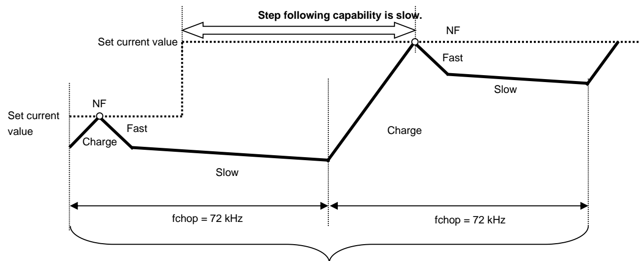
Figure 4.3 Chopping frequency (72 kHz)
