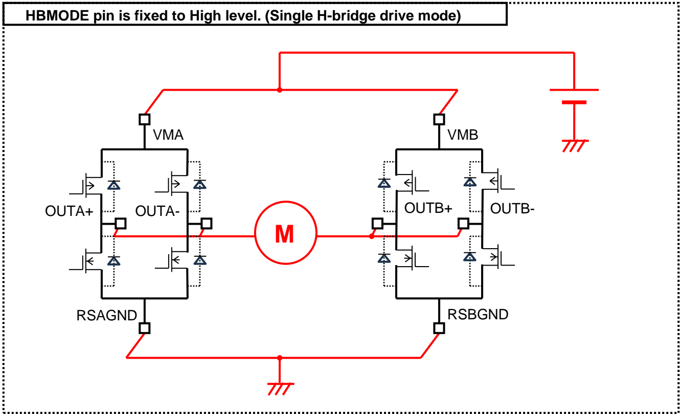
Figure 6.3 Connection example (Single H-bridge drive mode)
