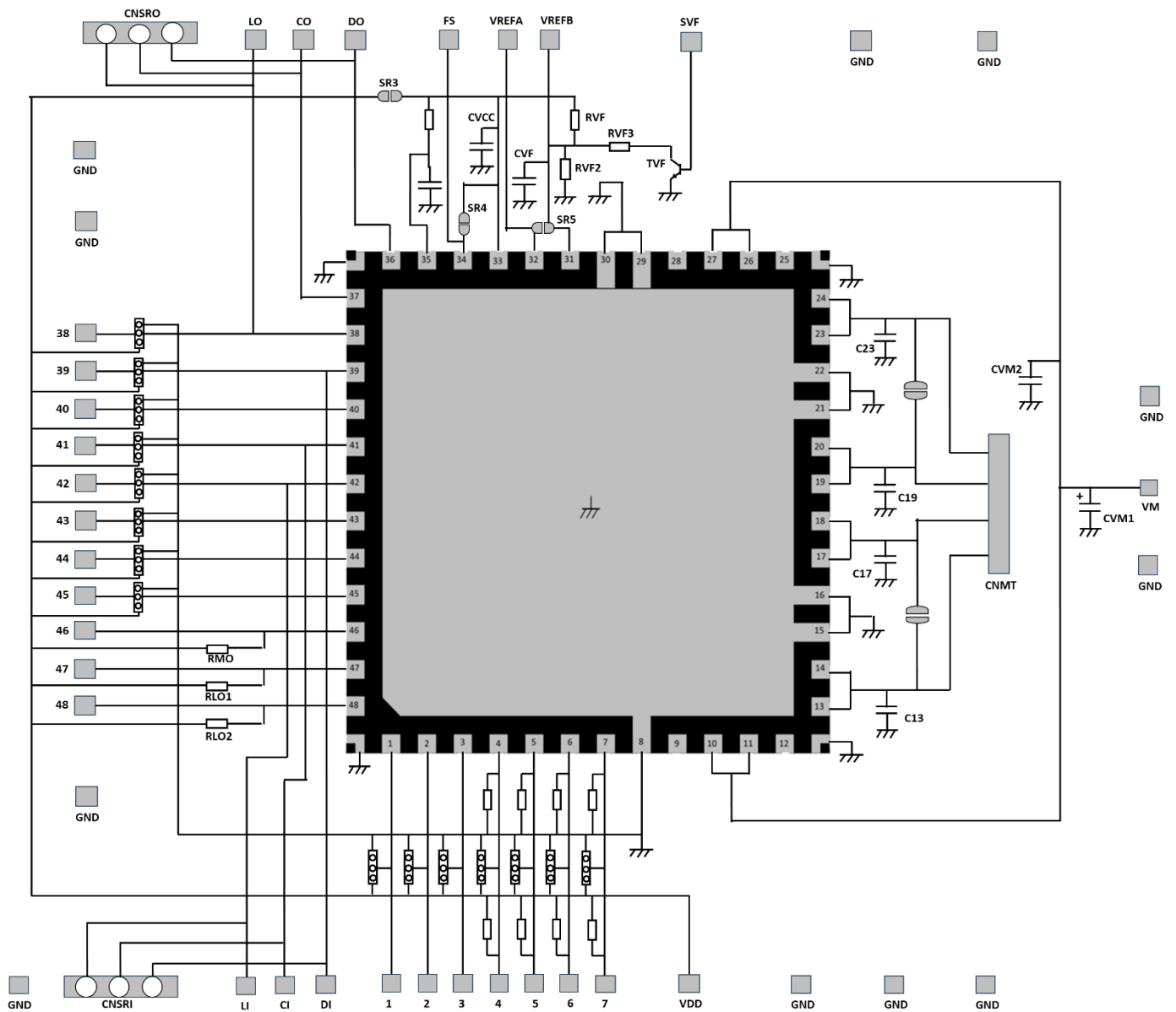
Figure 11.4 Board circuit diagram
