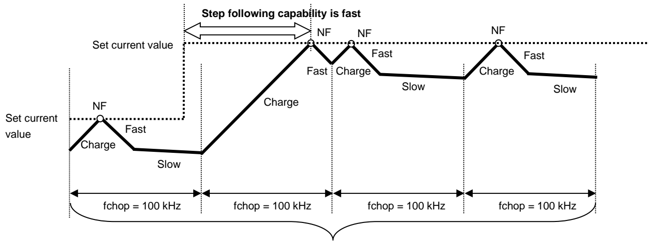
Figure 4.2 Chopping frequency (100 kHz)
