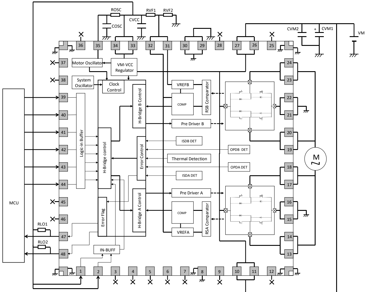
Figure 7.1 Application circuit example
