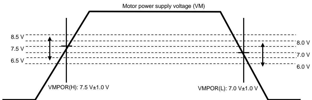
Figure 1.1 Power supply sequence and POR detection threshold
