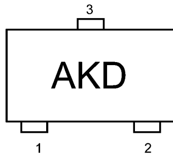
Fig. 8.1 Marking
