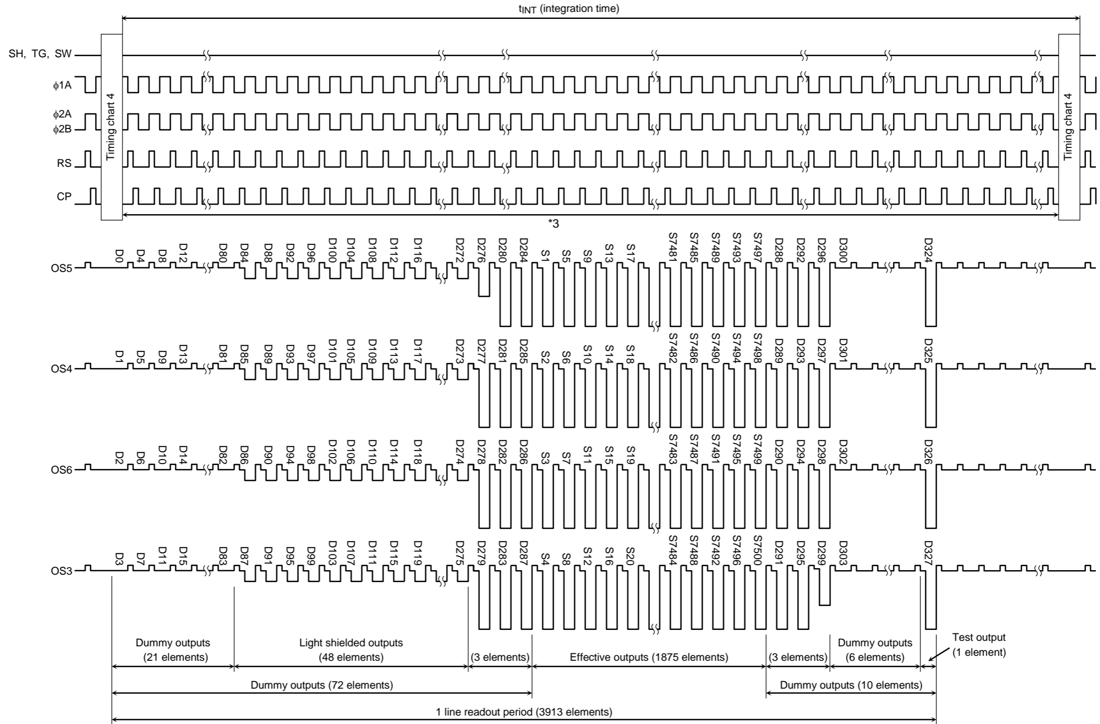
Timing Chart 3: B/W Mode (Refer to the Timing Chart 4)
