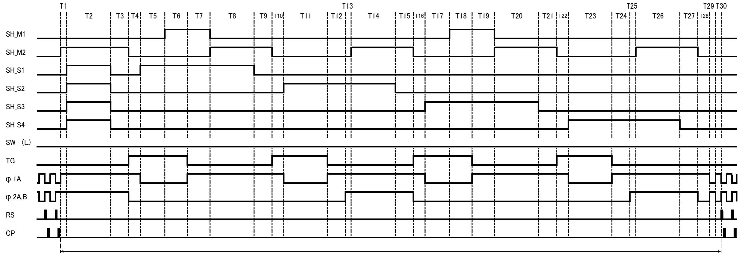
Timing Chart 4: B/W Mode (Vertical Transfer Period)
