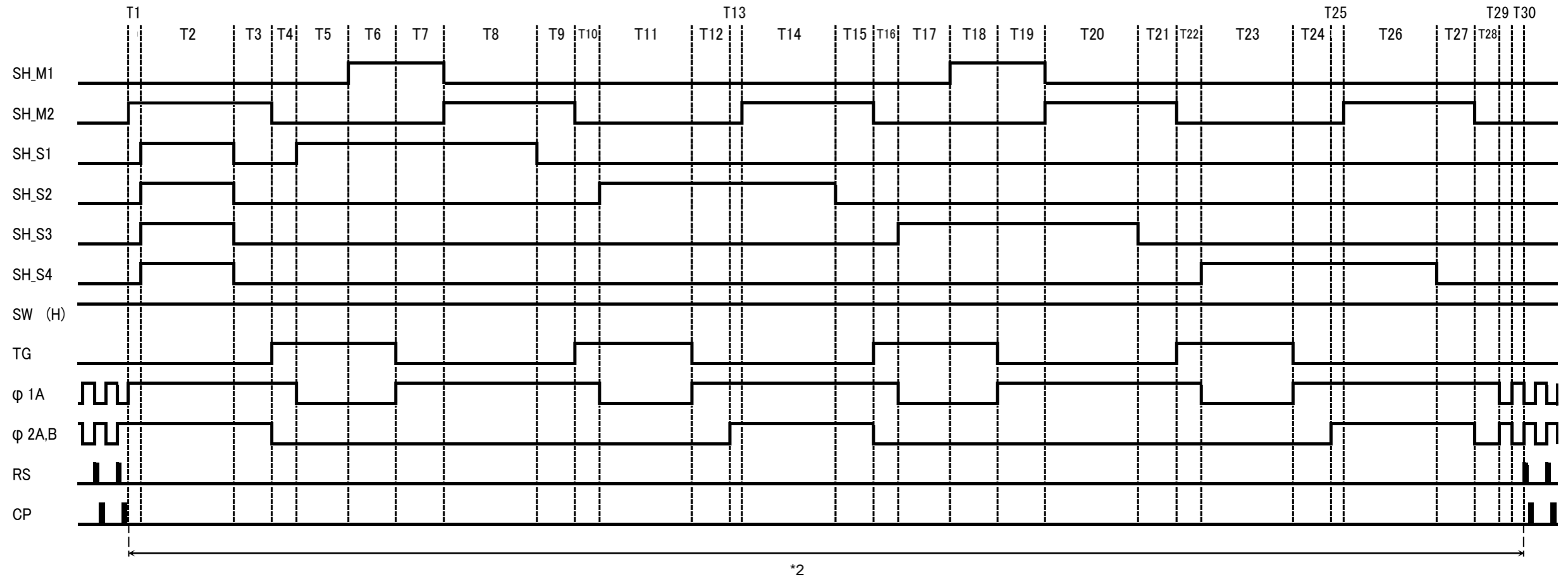
Timing Chart 2: Color Mode (Vertical Transfer Period)
