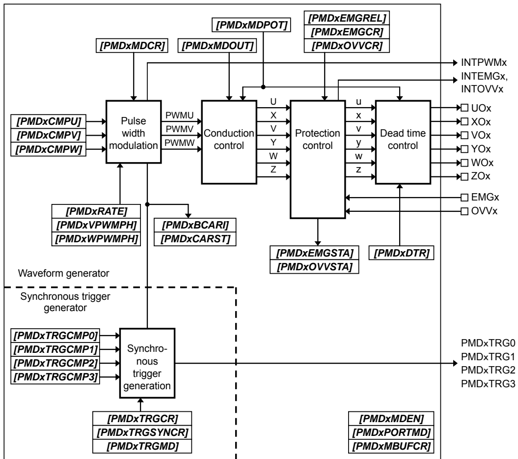
Figure 2.1 Block diagram of PMD circuit
