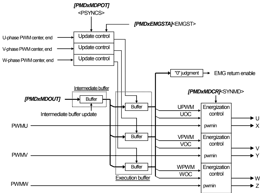
Figure 3.7 Conduction control circuit
