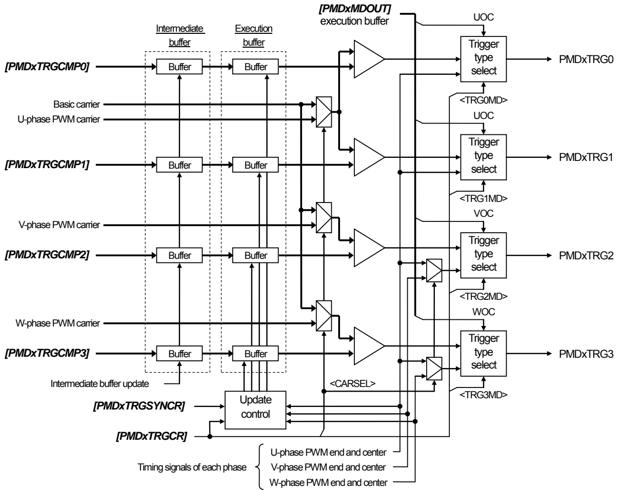
Figure 3.14 Synchronous trigger generation circuit
