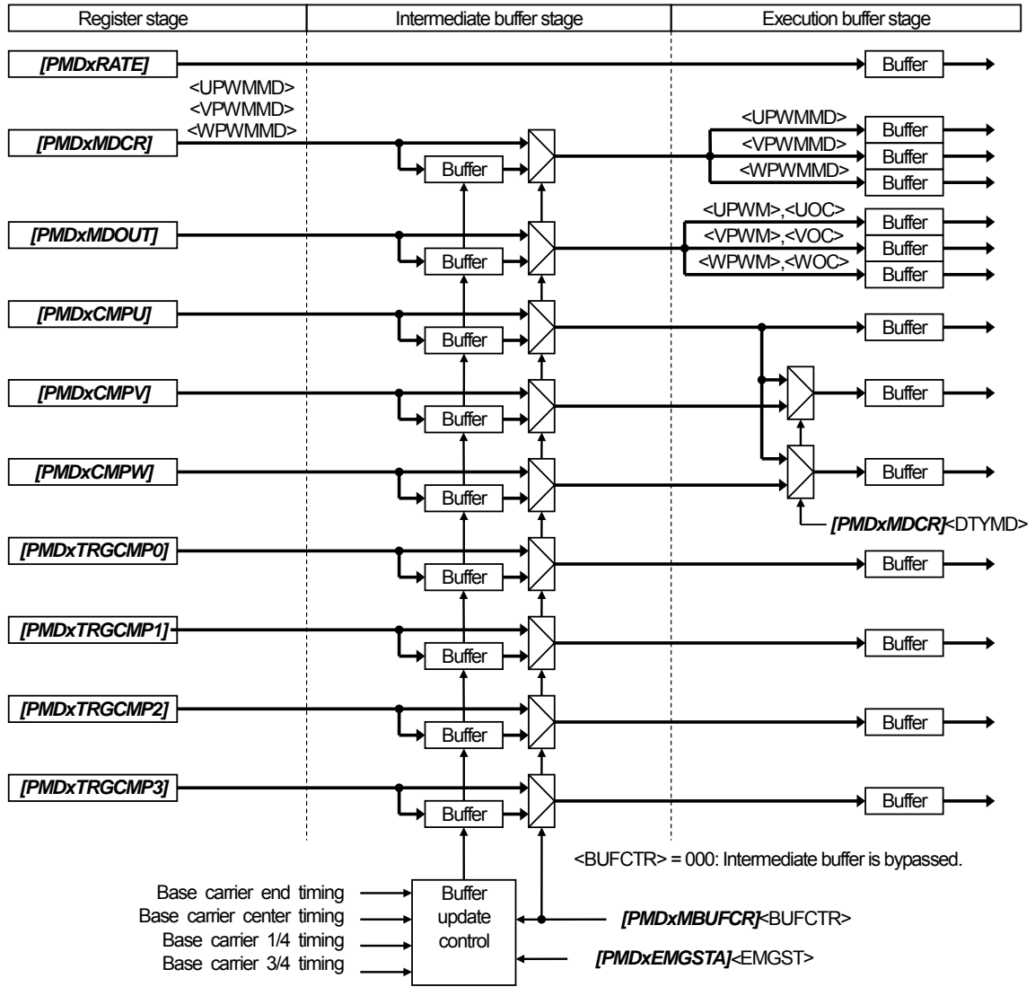
Figure 3.16 Register buffer configuration
