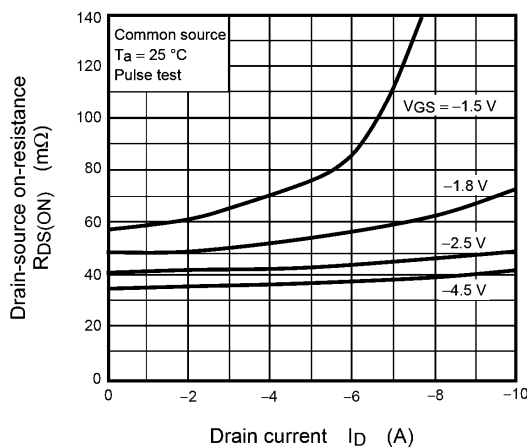
Fig. 7.5 R_{DS(ON)} - I_D
