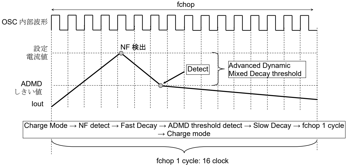
図 8.14 ADMD (Advanced Dynamic Mixed Decay) 定電流制御
