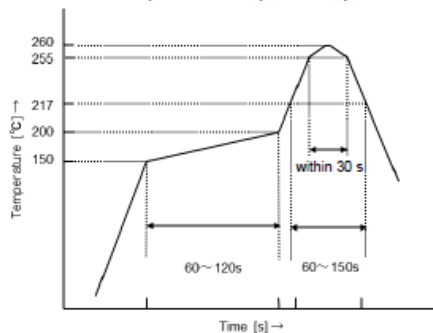
Figure 5 Typical package temperature profile
