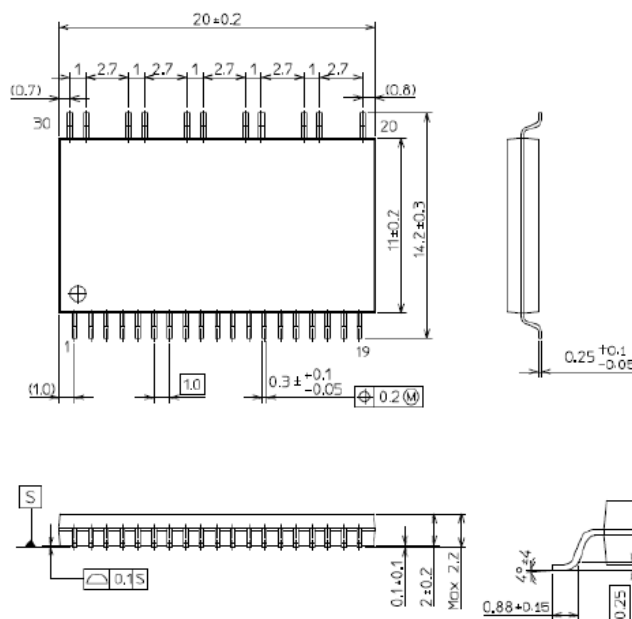
Figure 3 P-SSOP30-1120-1.00-001
