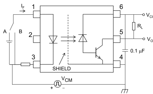
Fig. 13.1.6 Common-Mode Transient Immunity Test Circuit and Waveform
