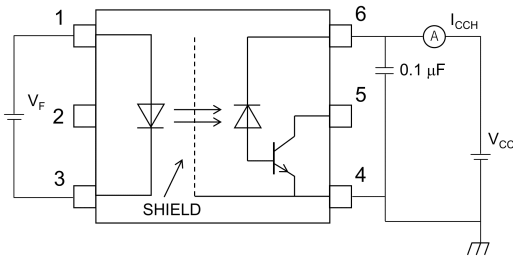
Fig. 13.1.3 ICCH Test Circuit
