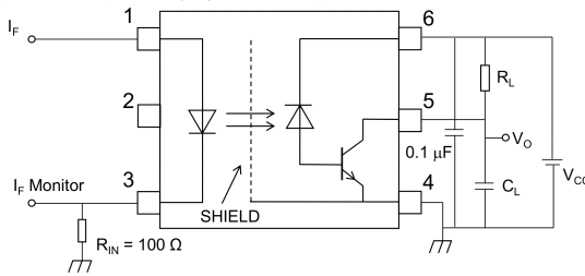
Fig. 13.1.5 Switching Time Test Circuit and Waveform
