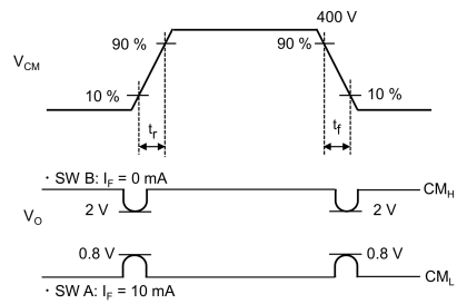
Fig. 13.1.5 Switching Time Test Circuit and Waveform
