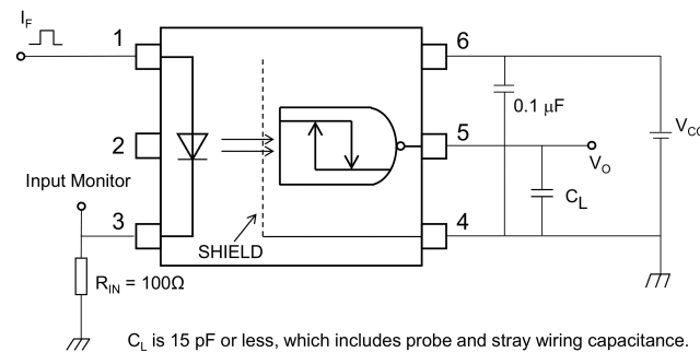
Fig. 14.1.5 Switching Time Test Circuit and Waveform
