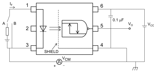
Fig. 14.1.6 Common-Mode Transient Immunity Test Circuit and Waveform
