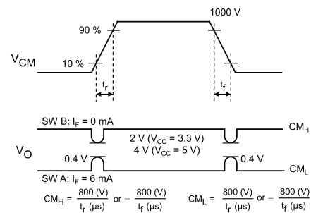
Fig. 14.1.6 Common-Mode Transient Immunity Test Circuit and Waveform
