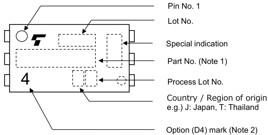
Fig. 18.4 Marking Example
