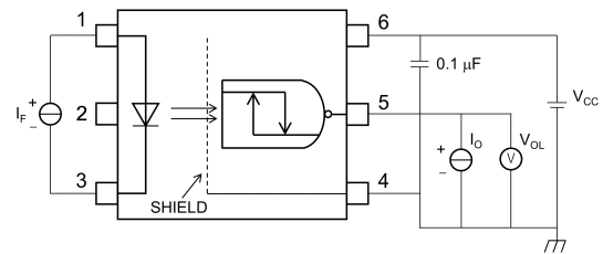
Fig. 14.1.2 V_{OL} Test Circuit
