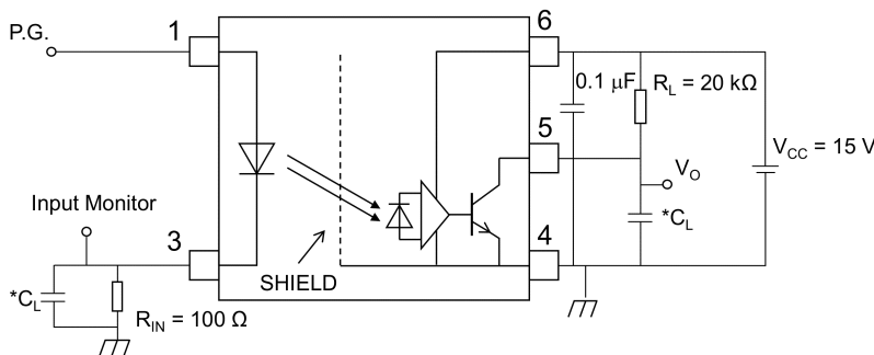
Fig. 12.1.6 Switching Time Test Circuit and Waveform
