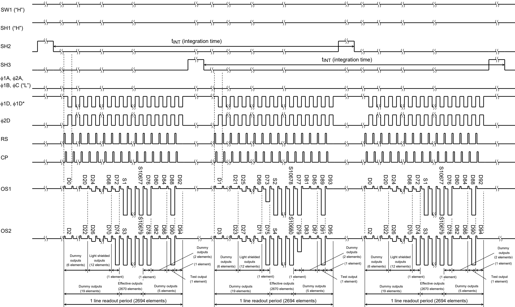
Timing Chart 5: B/W 1200 dpi Mode (Bit Clamp Mode)
