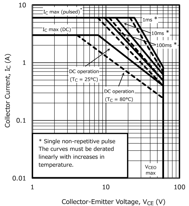
Figure 1.17 SOA for Transistor B and an example of SOA derated for T C = 80 °C
