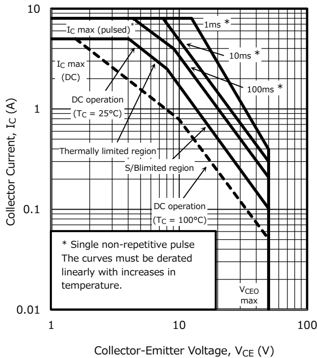
Figure 1.16 SOA for Transistor A and an example of SOA derated for T C = 100 °C
