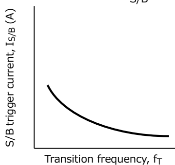
Figure 1.9 I_{S/B} vs. f_T
