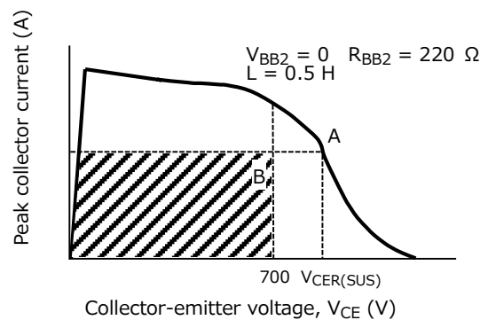
A peak collector current of 150 mA is applied, and the collector-emitter voltage at which the collector current drops to 100 mA is measured (A in the above figure).
