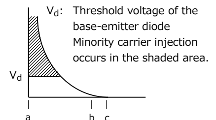
Figure 1.8 Base-emitter reverse bias
