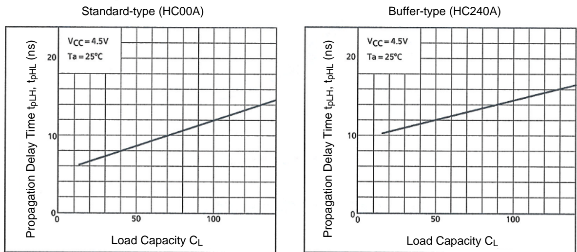
Figure 5.5 Dependence of Load Capacitance on t_{PLH} , t_{PHL}
