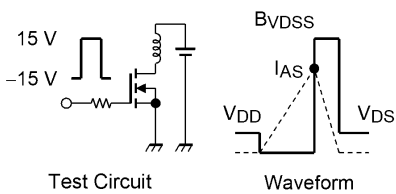
Fig. 8.16 Test Circuit/Waveform
