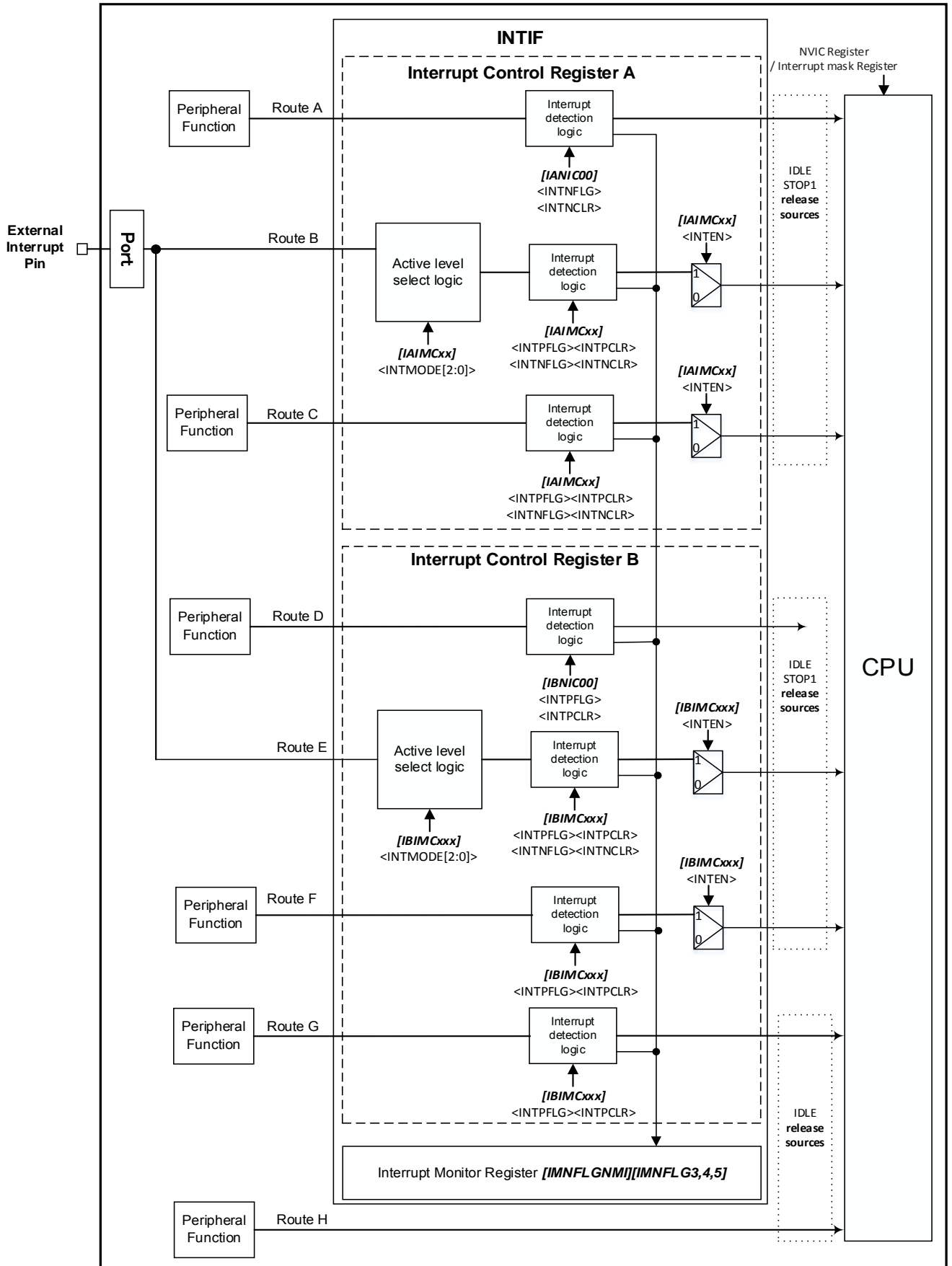
Figure 4.1 Interruption transfer route Diagram
