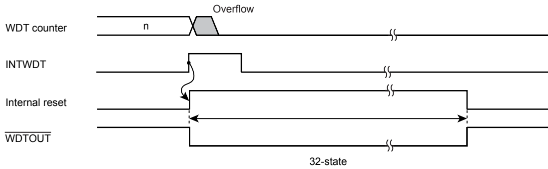
Figure 19-3 Internal reset generation
