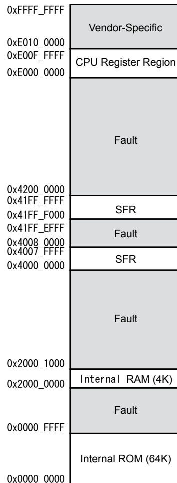
Figure 3-1 Memory Map
