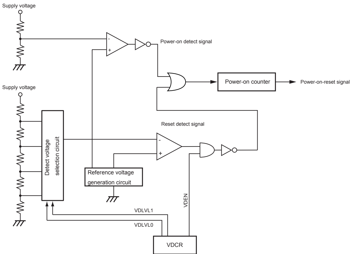
Figure 16-1 Power-on-reset circuit
