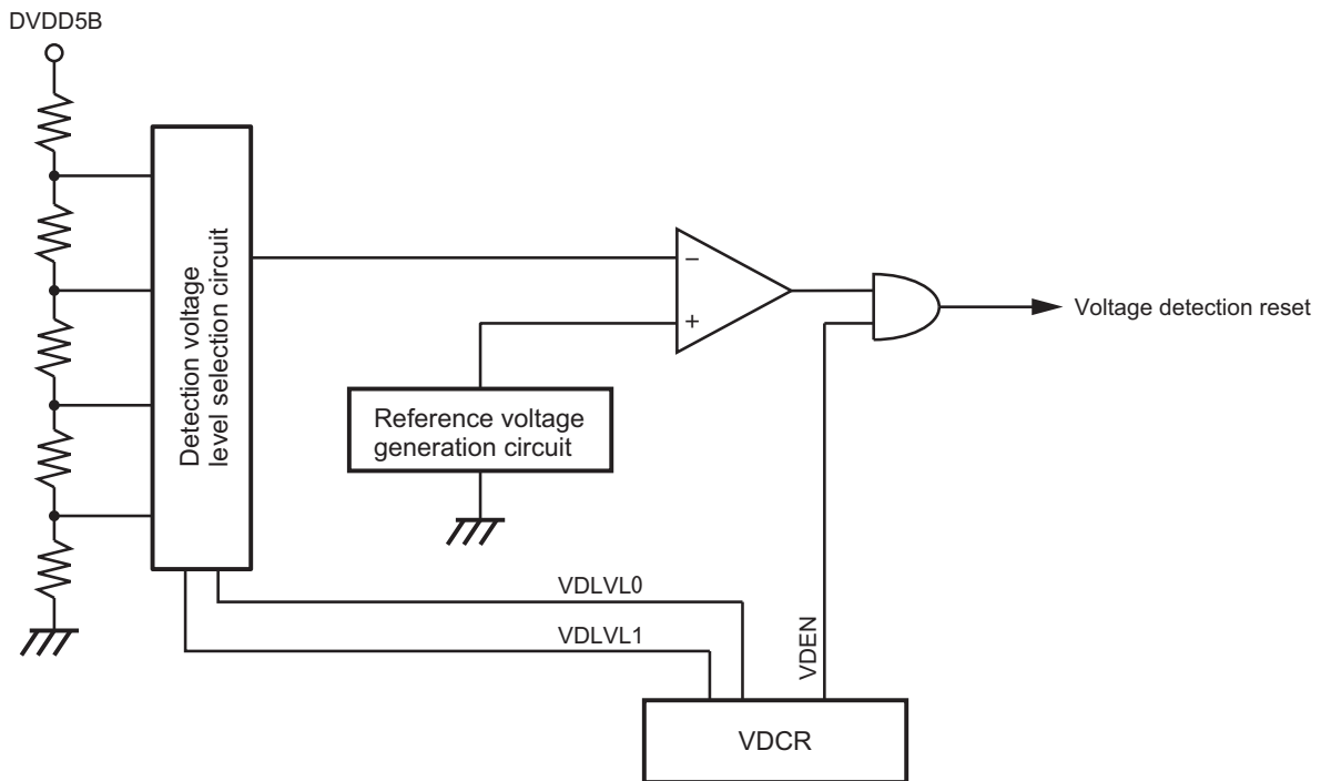
Figure 17-1 Voltage Detection Circuit
