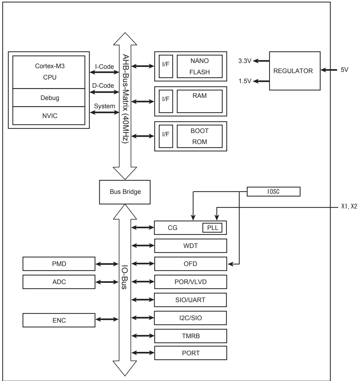
Figure 1-1 TMPM3U0FSDMG block diagram
