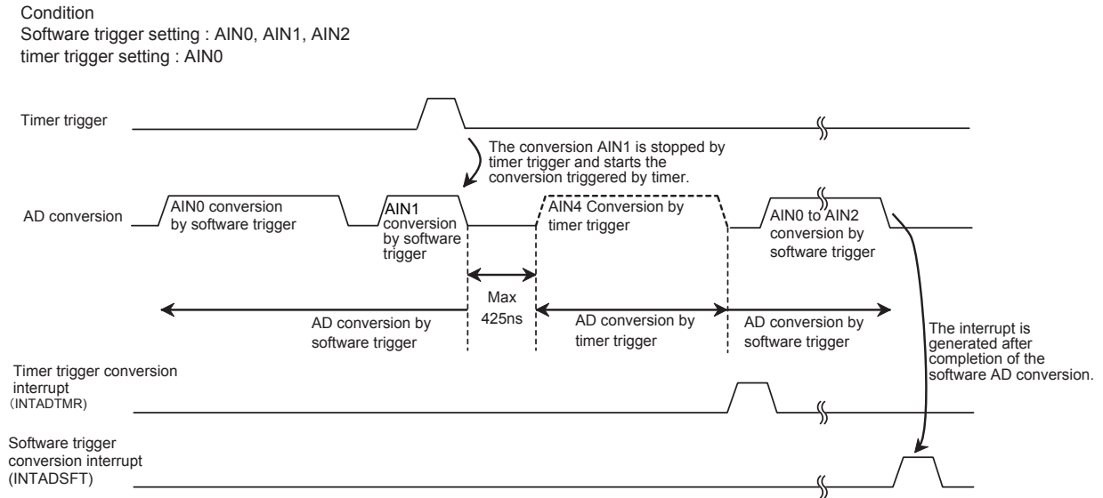
Figure 13-8 AD conversion by timer trigger
