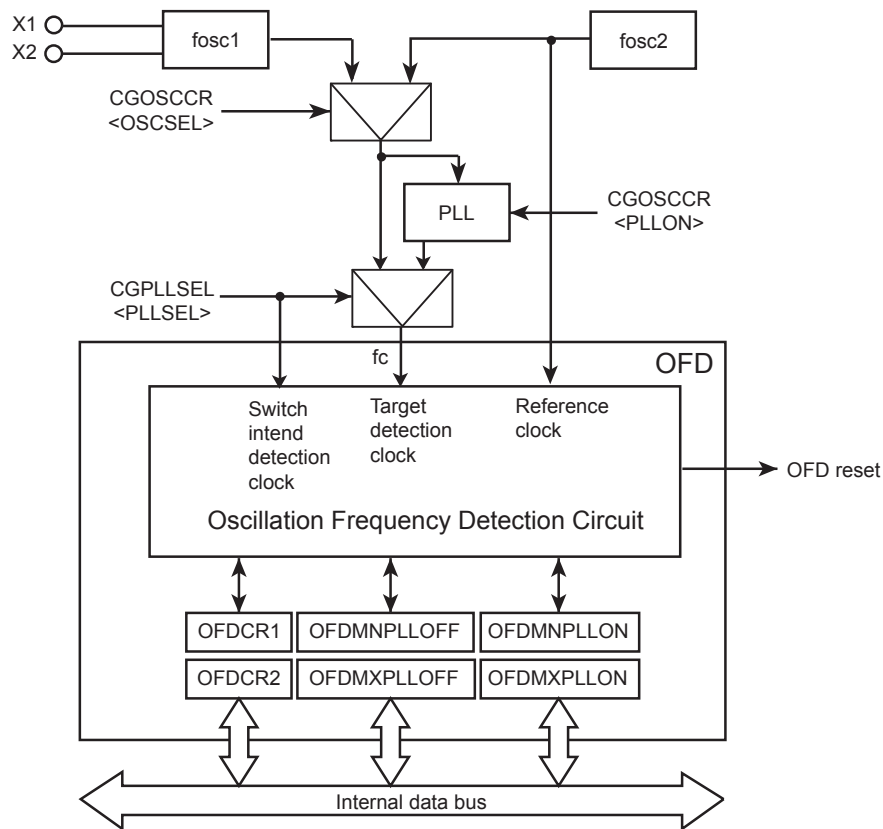
Figure 18-1 Oscillation Frequency Detector Block diagram
