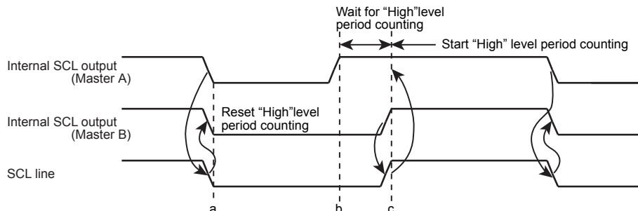
Figure 12-4 Example of Clock Synchronization
