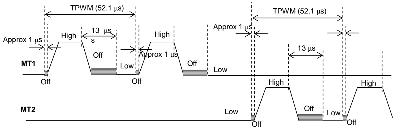
Figure 7.26 PWM Waveforms
