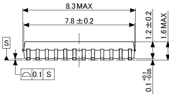
Figure 12.1 Package Dimensions
