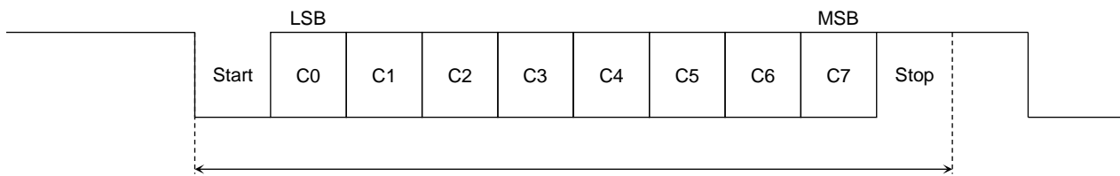
Figure 7.20 Checksum Field
