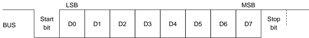
Figure 7.4 DATA Frame
