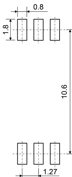
Fig. 15.1 Lead forming and taping option (LF4), (TP4)
