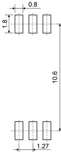
Fig. 15.1 Lead forming and taping option (LF4), (TP4)
