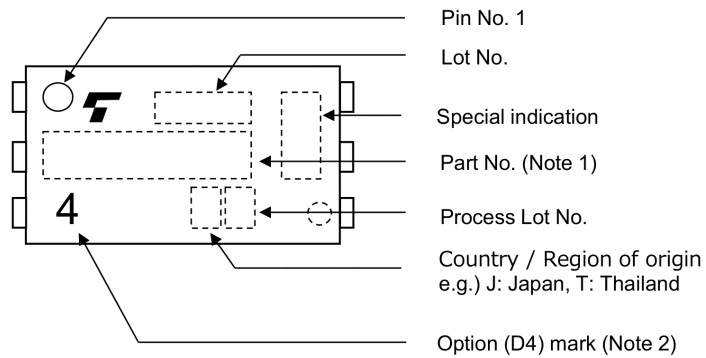
Fig. 17.3 Marking Example
