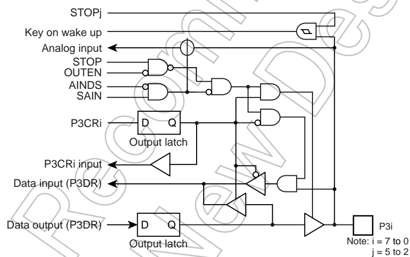
Figure 5-5 Port P3
