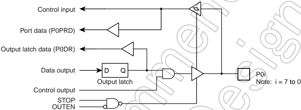
Figure 5-2 Port 0
