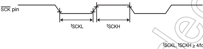
Figure 10-3 External Clock
