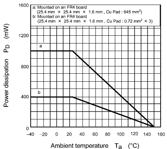
Fig. 8.12 P_D - T_a
