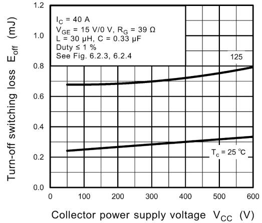
Fig. 8.14 E_{off} - V_{CC}
