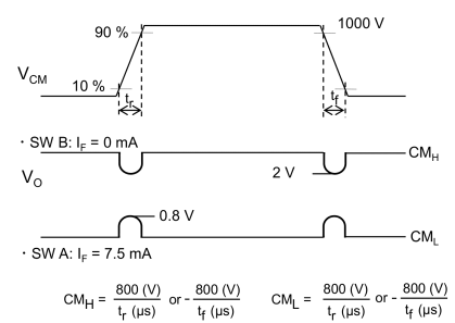
Fig. 12.1.6 Common-Mode Transient Immunity Test Circuit and Waveform
