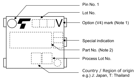
Fig. 16.4 Marking Example
