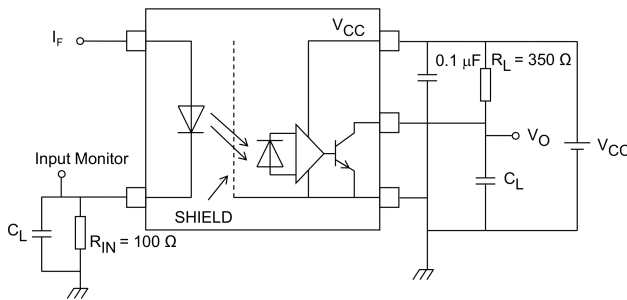
Fig. 12.1.5 Switching Time Test Circuit and Waveform
