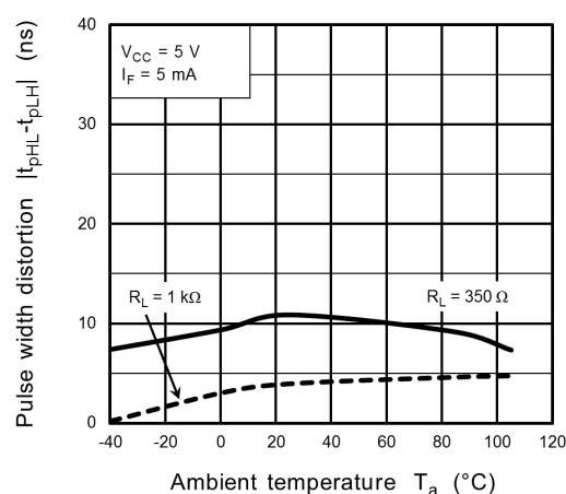
Fig. 12.2.18 |t_{pHL} - t_{pLH}| - T_a
