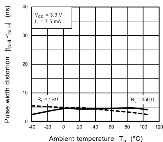
Fig. 12.2.16 |t_{pHL} - t_{pLH}| - T_a
