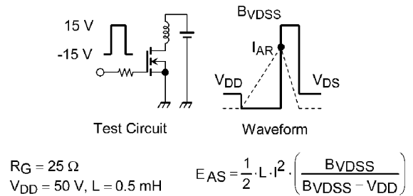
Fig. 8.16 Test Circuit/Waveform
