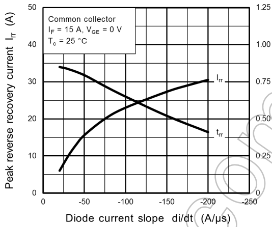
Fig. 8.15 I_{rr}, t_{rr} - di/dt
