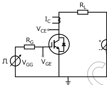
Fig. 6.2.1 Test Circuit of Switching Time
