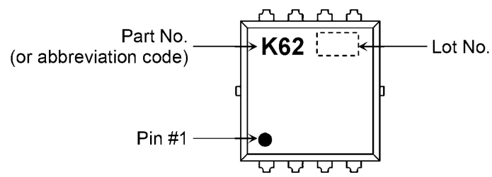
Fig. 7.1 Marking
