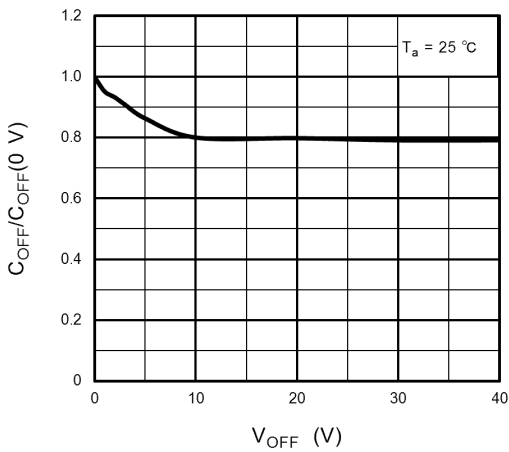
図 12.1.11 C_{OFF}/C_{OFF(0V)} - V_{OFF}
