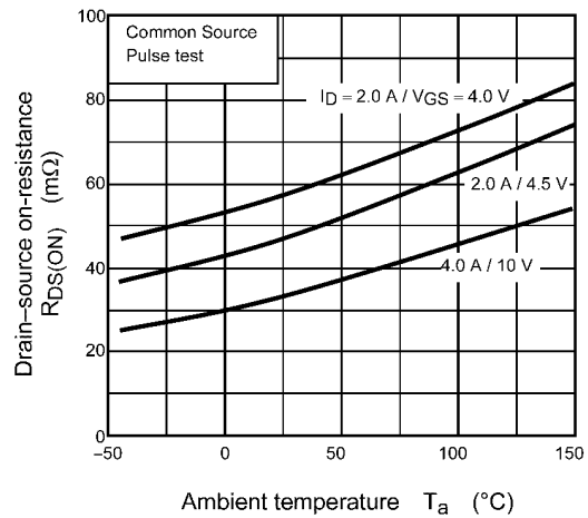
Fig. 8.6 R_{DS(ON)} - T_a
