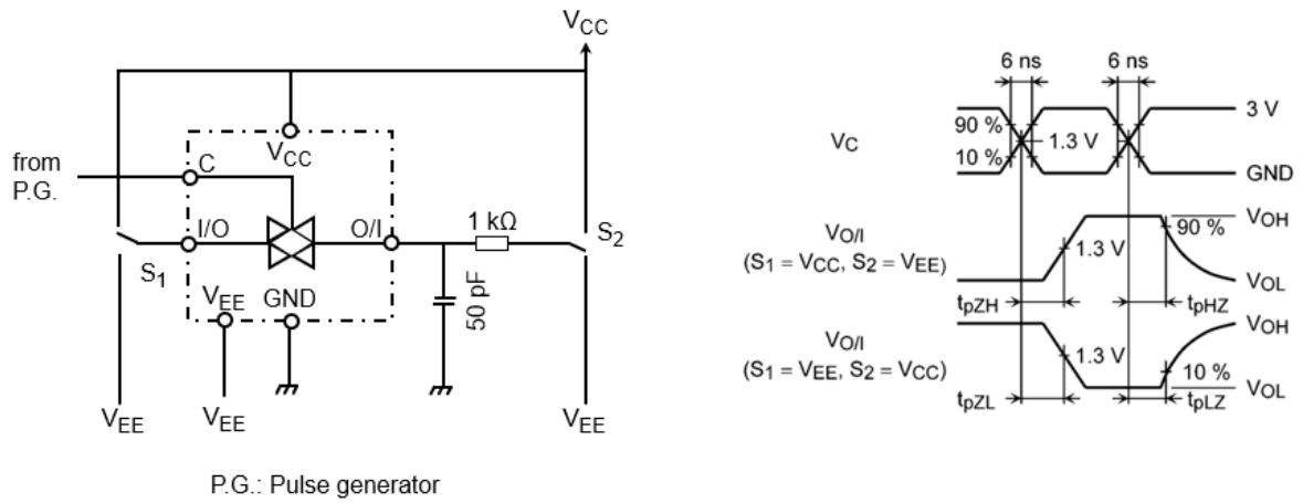
図1. t_{pLZ} , t_{pHZ} , t_{pZL} , t_{pZH}
