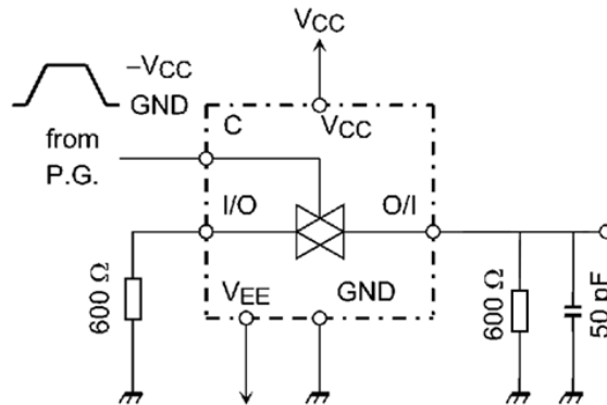
图4. Feedthrough Attenuation
