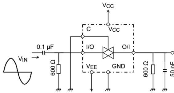
图4. Feedthrough Attenuation
