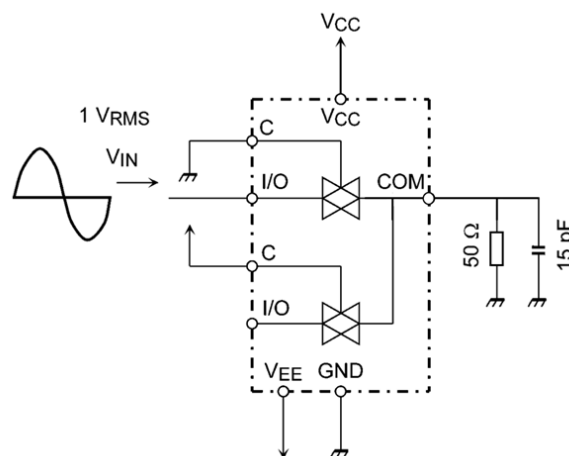
图6. Cross Talk (between any two switches)
