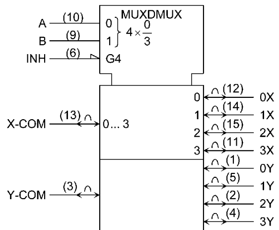
74HC4052FT
