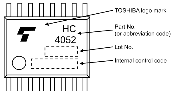
74HC4052FT
