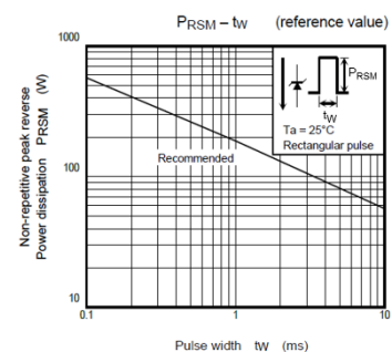
Figure 3.4 Example of surge power tolerance
