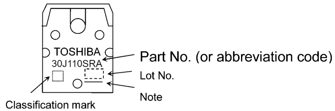
Fig. 7.1 Marking
