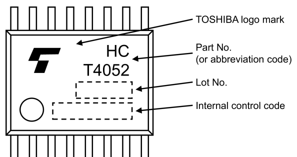
74HCT4052FT
