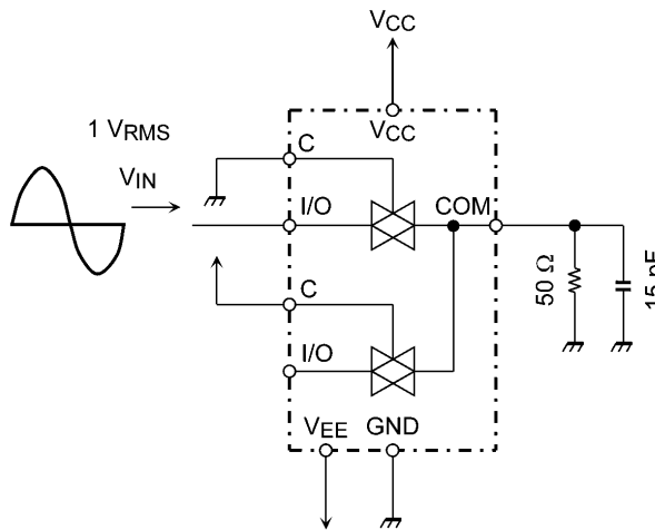
图6. Cross Talk (between any two switches)
