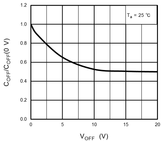
C_{OFF}/C_{OFF}(0\text{ V}) - V_{OFF}
