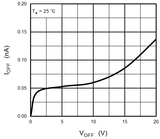
IOFF - VOFF
