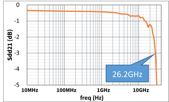
Frequency Characteristics of Toshiba High-Speed Bus Switches (Toshiba TDS4B212MX)
