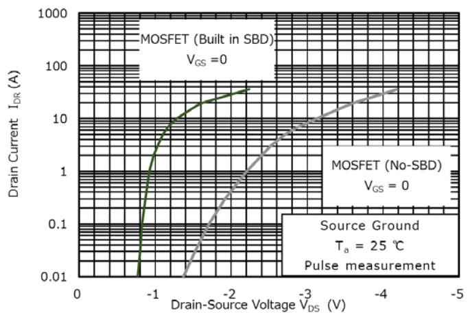
Figure 6. I_{DR} - V_{DS} Characteristics
