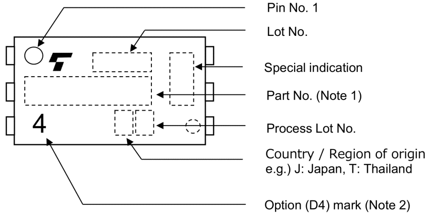
Fig. 17.4 Marking Example
