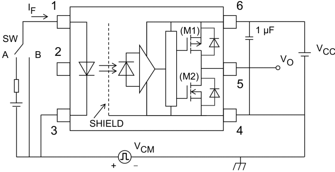
Fig. 13.1.8 Common-Mode Transient Immunity Test Circuit and Waveform
