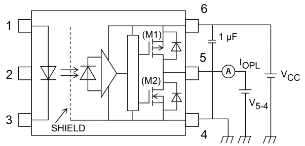
Fig. 13.1.2 I_{OPL} Test Circuit
