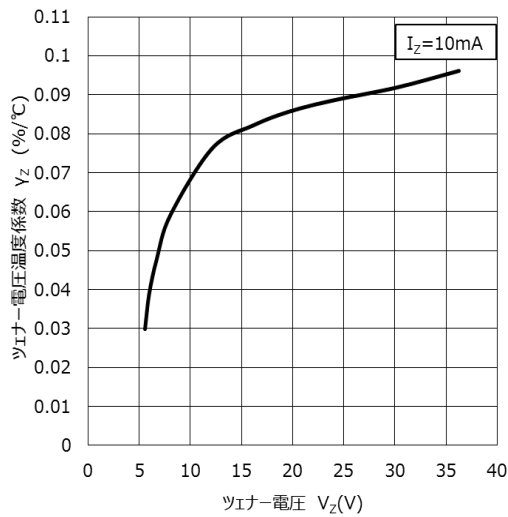
\gamma_z - V_z
