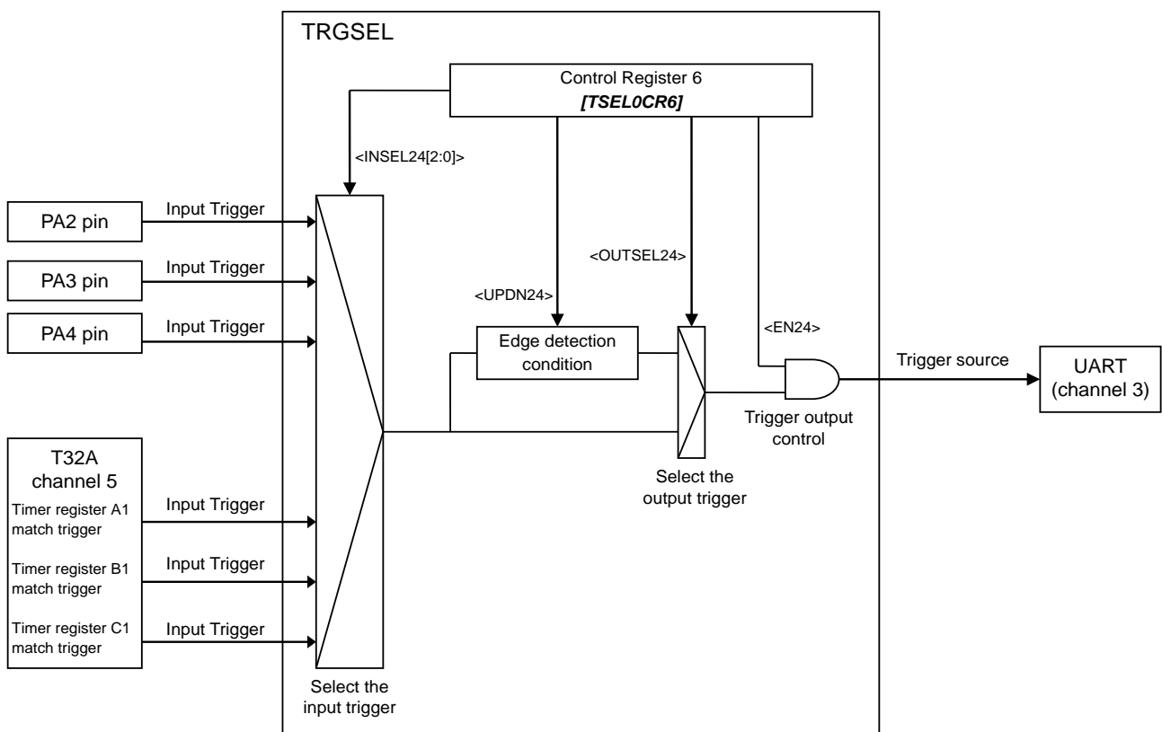
Figure 2.1 Example of Trigger Selector Connection
