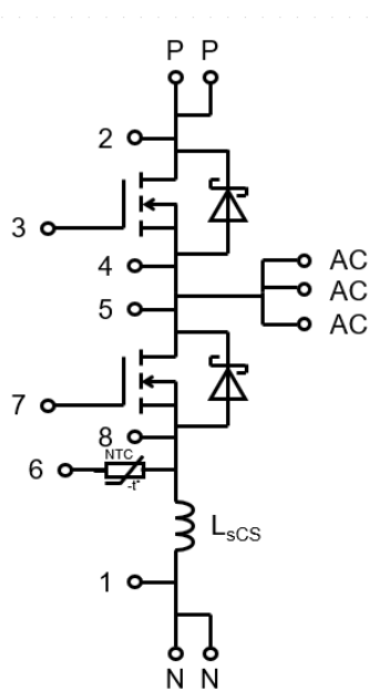
Figure 1.2.1 Internal circuit
