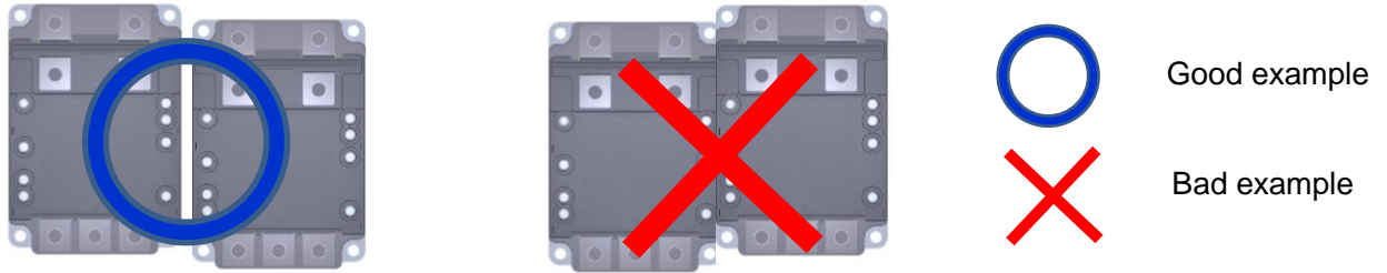
Figure 2.4.1.1 Mounting design on a heatsink
