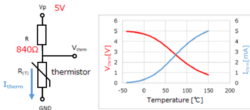
Figure 1.3.2 An example of the circuit and output voltage and current for a thermistor
