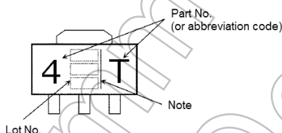
Fig. 6.1 Marking (Note)
