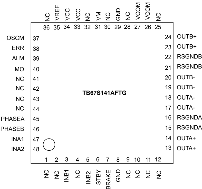
Figure 4.1 Pin Assignments (top view)
