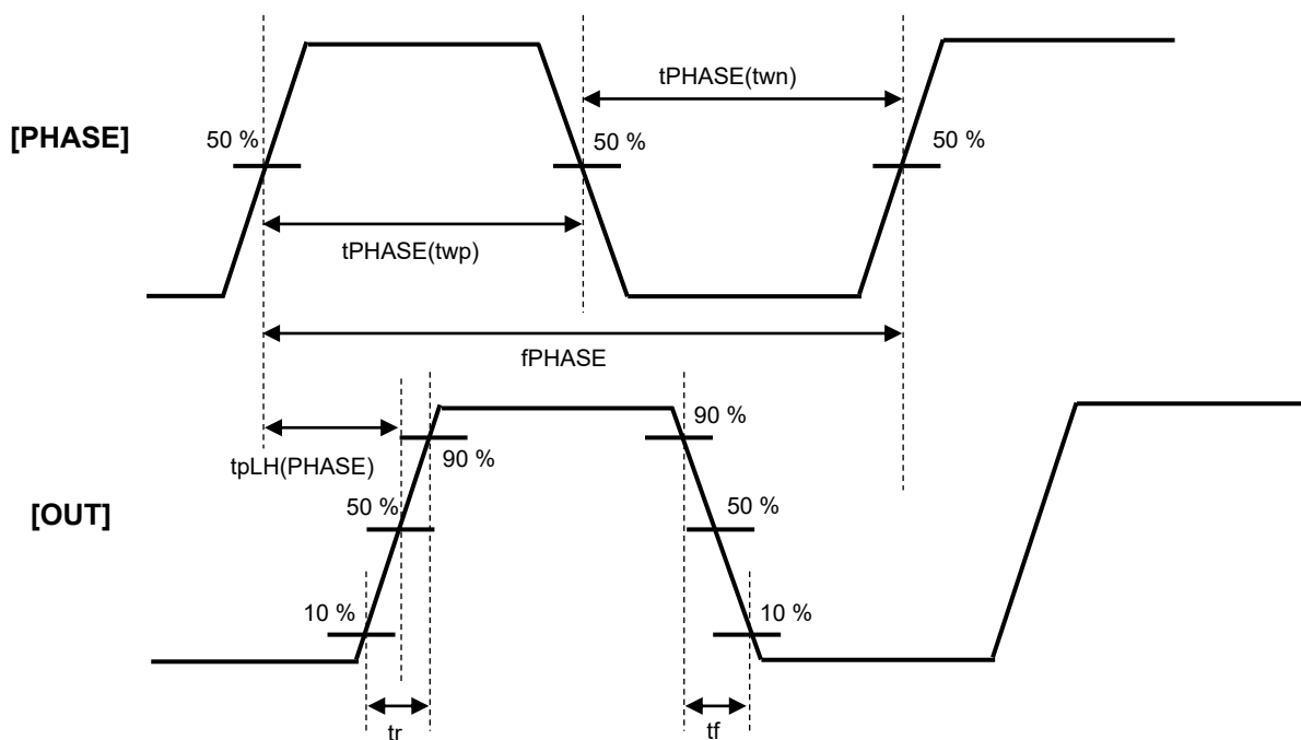
Figure 9.1 AC Timing chart
