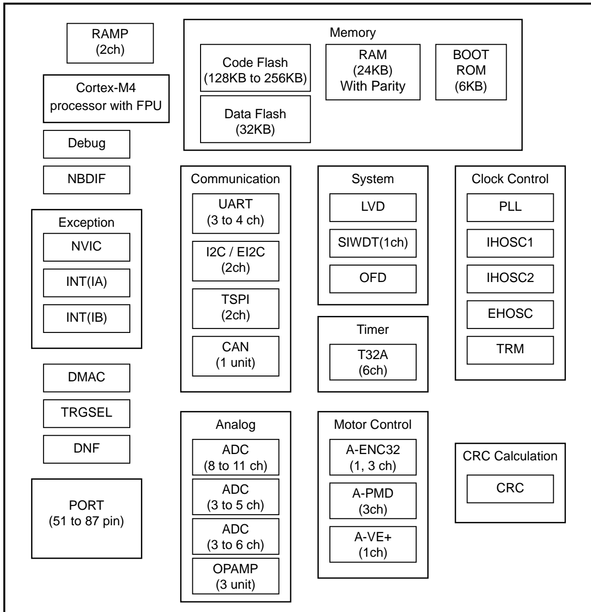
Figure 1.1 Block diagram of the TMPM4M Group(1) products
