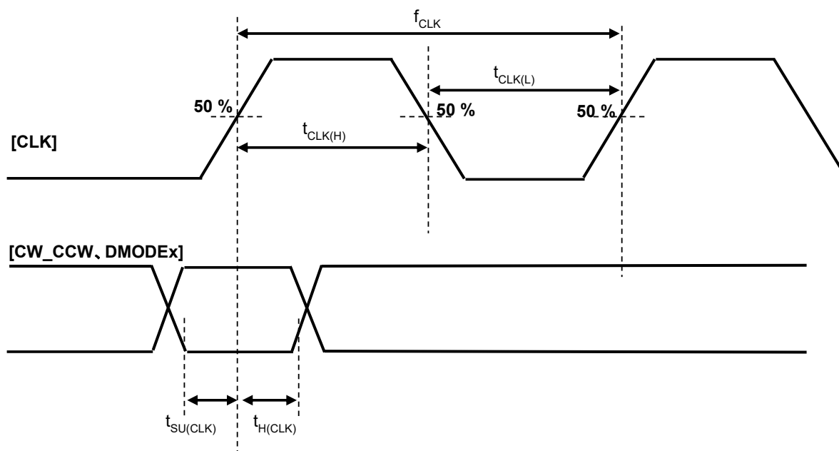
Figure9.2 TB67S539FTG(Relationship between CLK and other control signals)
