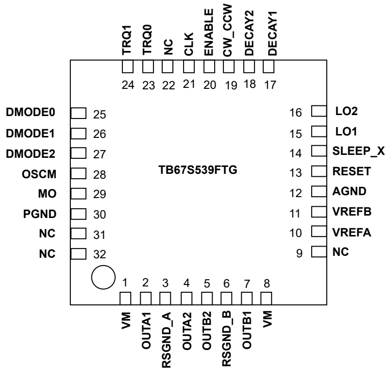
Figure 4.1 Pin Assignments
