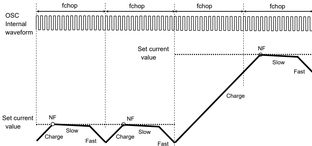
Figure 6.13 When the Charge period is more than 1 f_{CHOP} cycle
