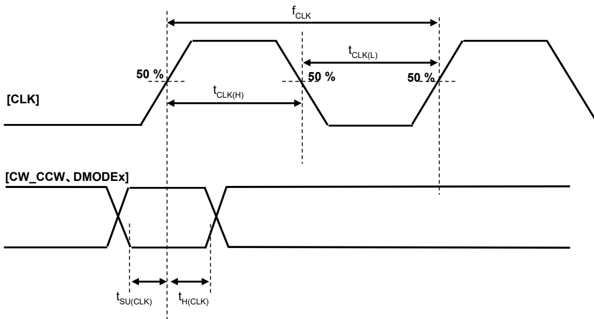
Figure9.2 TB67S539FTG(Relationship between CLK and other control signals)
