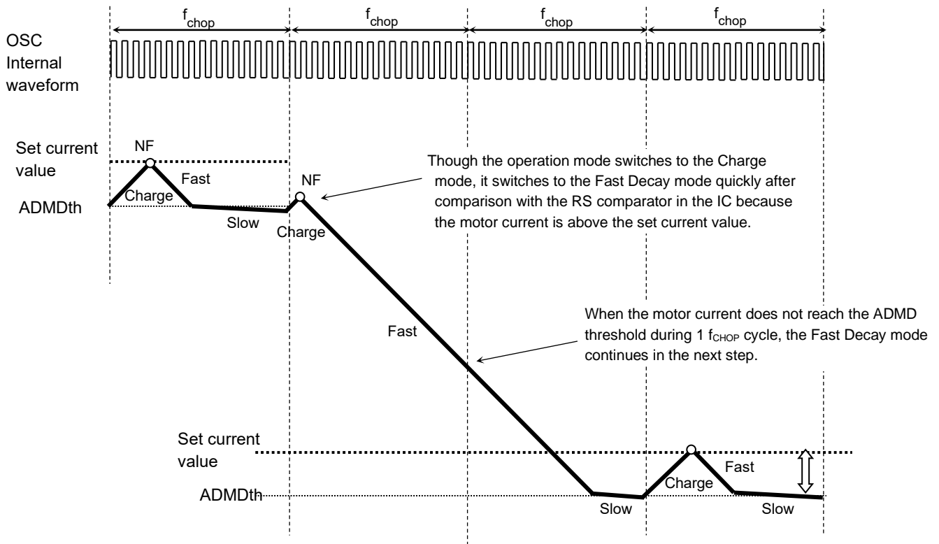
Figure 6.21 Fast period > 1 f_{CHOP} cycle
