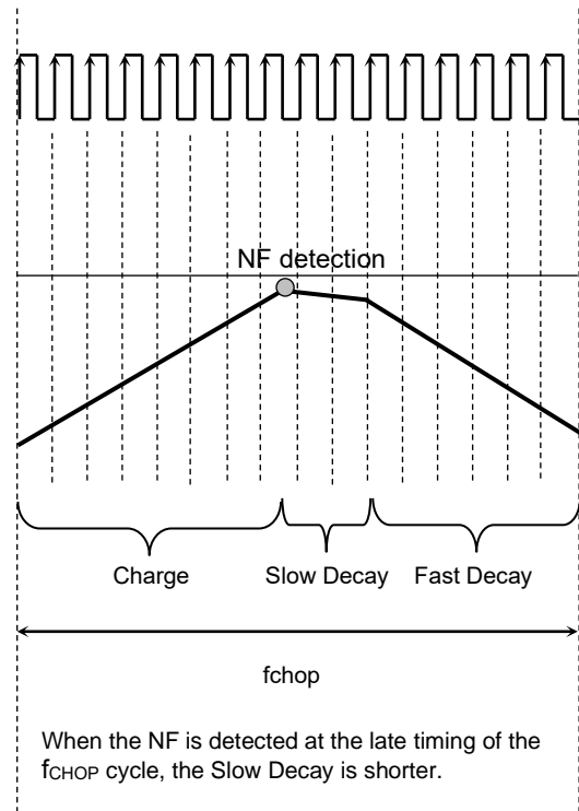
Figure 6.11 Each Time of Constant Current (2)
