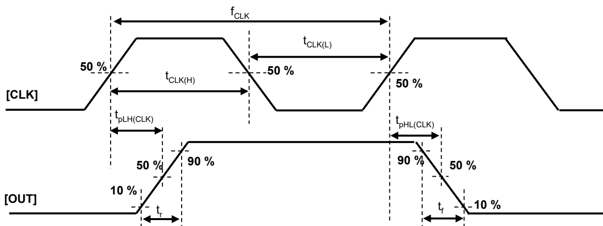
Figure9.1 TB67S539FTG(Relationship between CLK and output)
