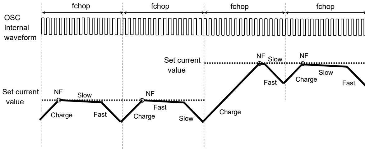
Figure 6.12 When the set current value is increased
