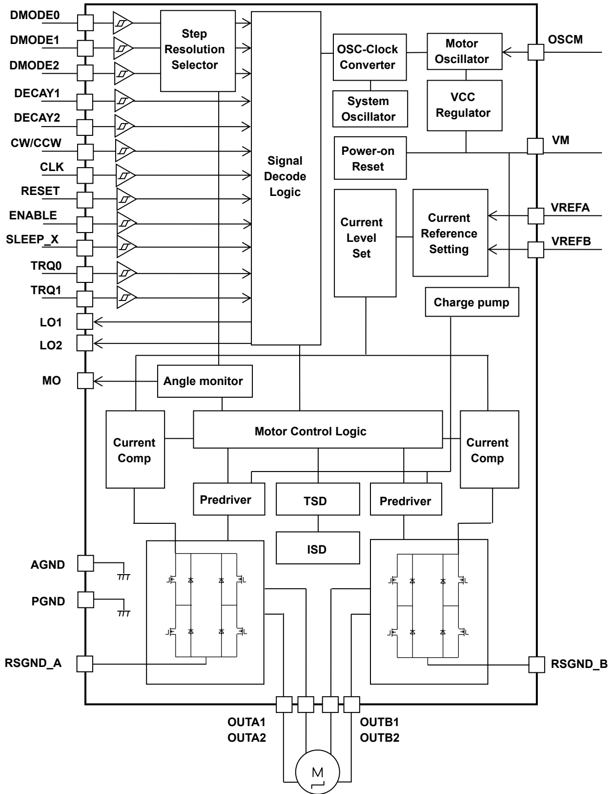
Figure 3.1 Block Diagram
