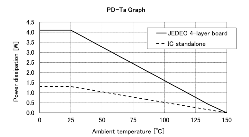
Figure7.1 PD-Ta graph
